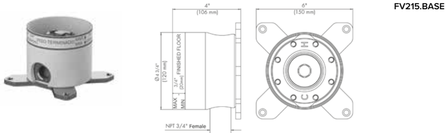
Freestanding rough valve 3/4" NPT FEM
